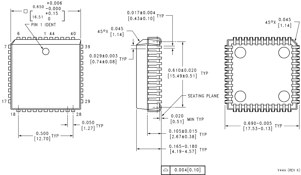
Plastic Leaded Chip Carrier (VA) Order Number COP8SBE9HVA7, COP8SCE9HVA7, COP8SDE9HVA7, COP8SCE9HVA9 or COP8SDE9HVA9 NS Package Number V44A
