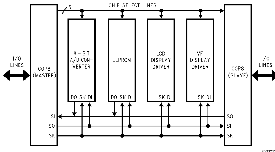
FIGURE 29. MICROWIRE/PLUS Application
